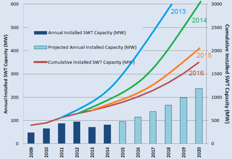
SWT Installed Capacity World Market Forecast 2009 - 2020
